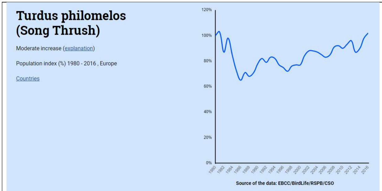
Figure 4: Long-term trend classification for Turdus philomelos . Source: EBCC (2018 update). Available at: https://pecbms.info/trends-and-indicators/species-trends/species/turdus-philomelos/ .
